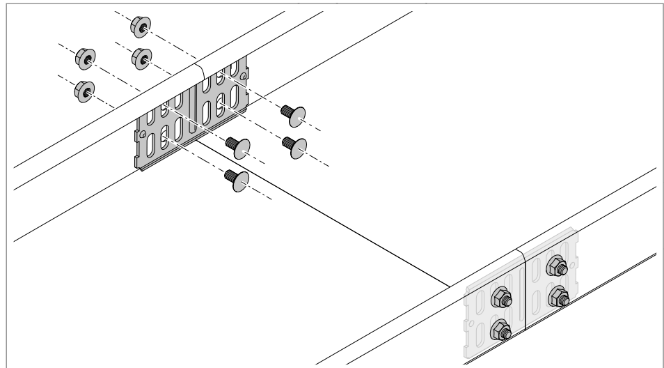
Figura 25: Aparafusar as uniões retas RLVK
