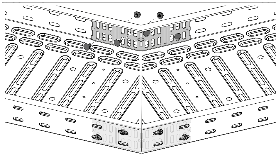
Figura 34: Aparafusar as uniões curvas RWVL
