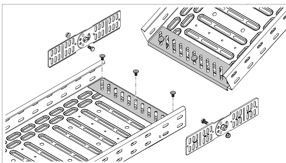
Figura 38: Aparafusar as placas de fundo
